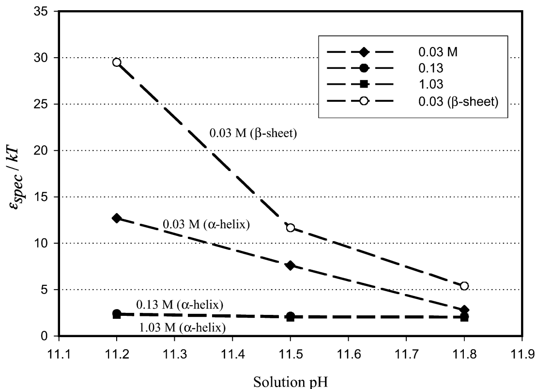
Fig. 4. Calculated values of \varepsilon_{\text{spec}}/kT for poly-L-lysine as a function of solution pH in aqueous NaCl solutions. Open symbols represent the \beta -sheet conformation and filled symbols represent the \alpha -helix conformation.
