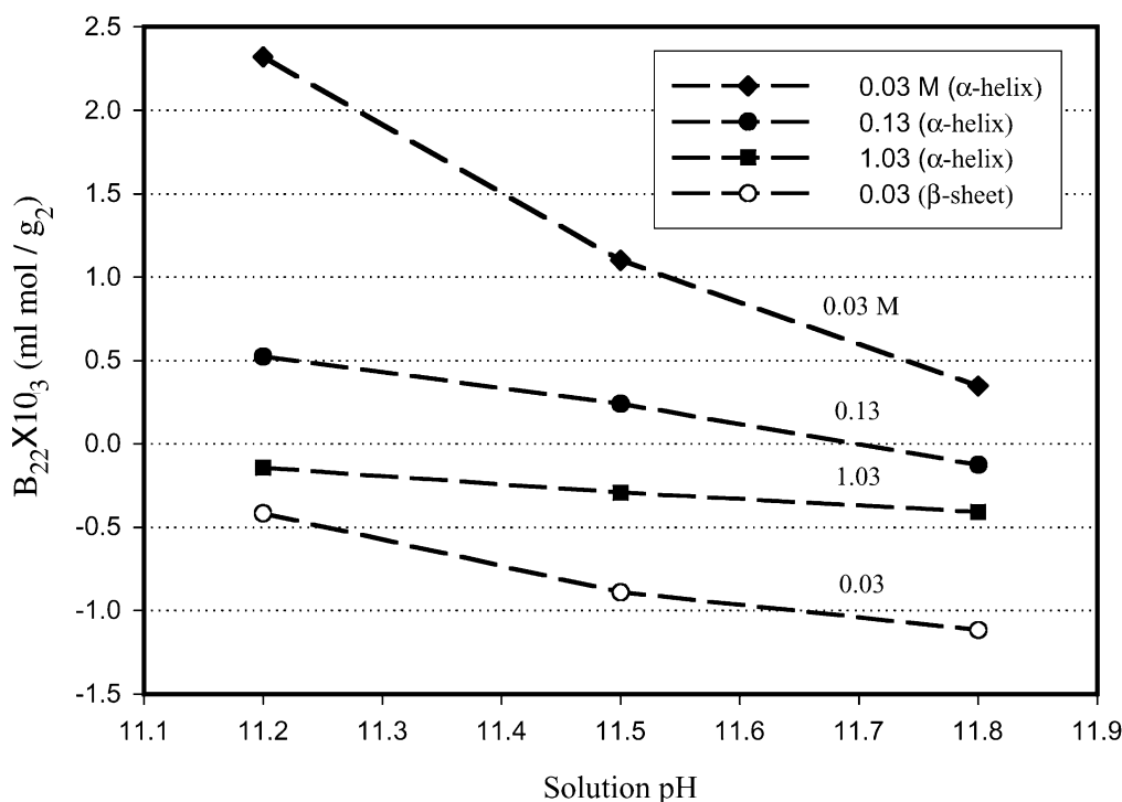
Fig. 3. Osmotic second virial coefficients ( B_{ave} ) as a function of solution pH determined by low-angle laser-light scattering for poly-L-lysine in aqueous NaCl solutions. Filled symbols represent PLL in the \alpha -helix conformation and open symbols ( \circ ) represent PLL in the \beta -sheet conformation.
