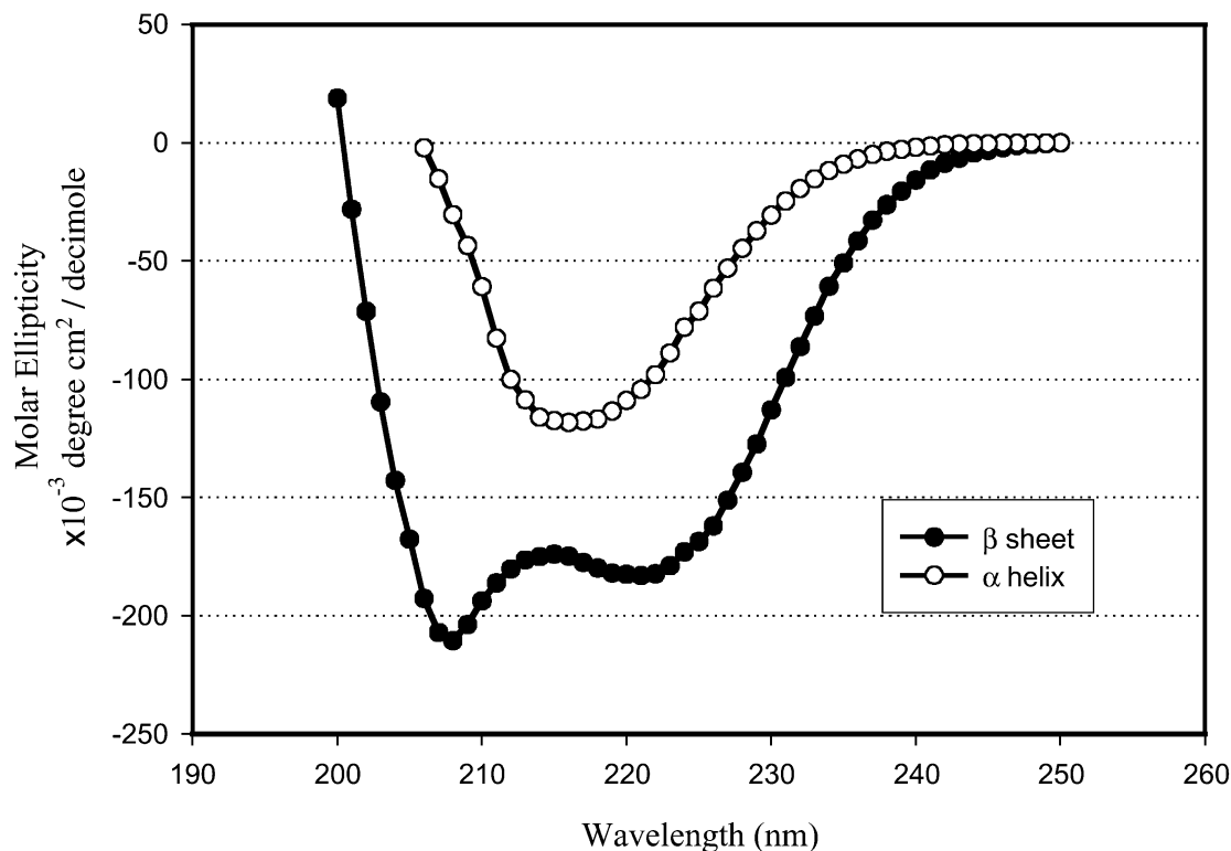
Fig. 1. Far-UV circular dichroism spectra of poly-L-lysine at pH 11.5 in 0.03 M aqueous NaCl solution in the \alpha -helix (●) and \beta -sheet (○) conformations.
