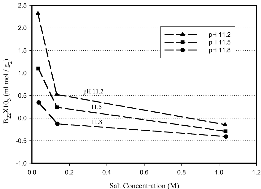
Fig. 2. Osmotic second virial coefficients ( B_{22} ) plotted as a function of NaCl concentration determined by low-angle laser-light scattering for poly-L-lysine in the \alpha -helix conformation.
